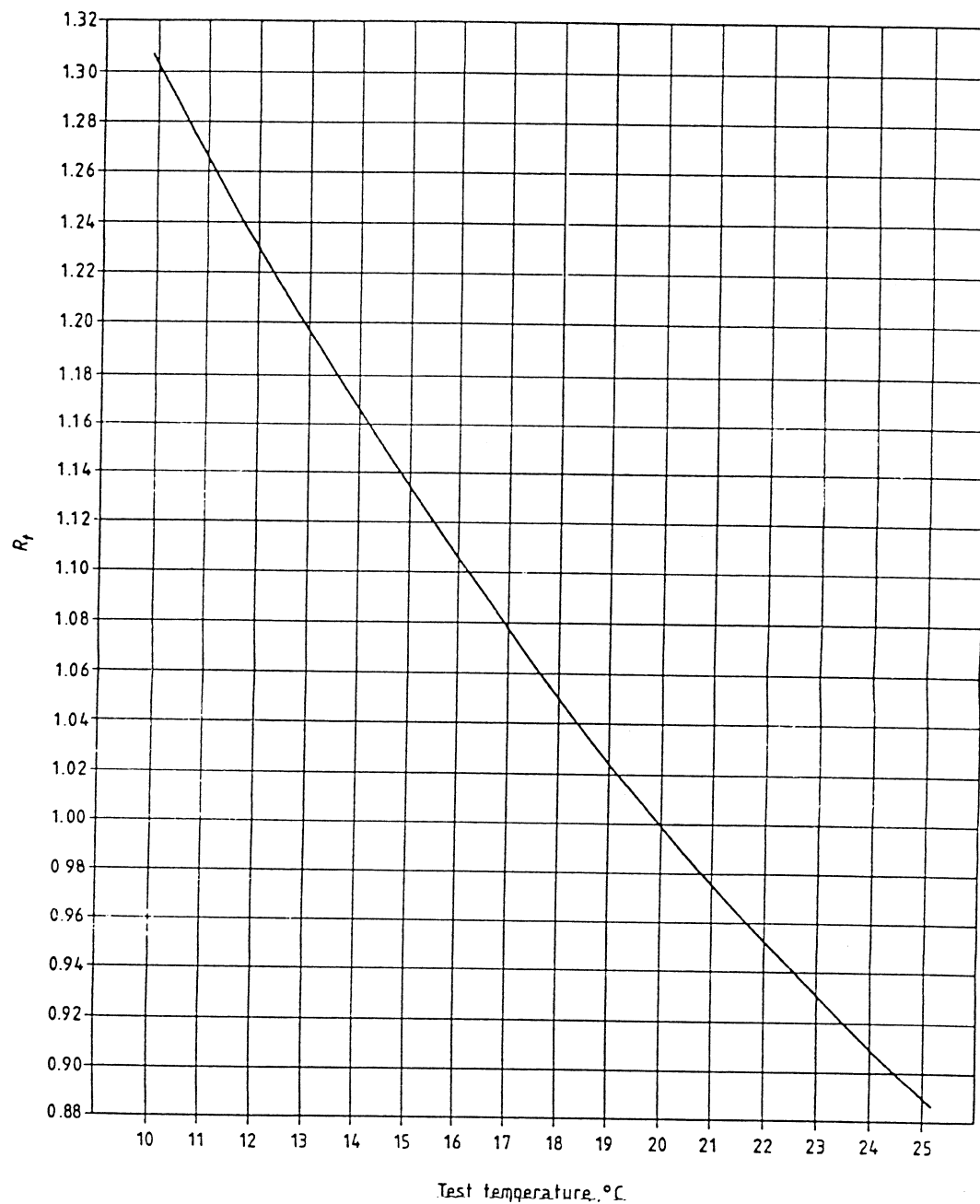
Figure 2 — Water viscosity correction factor R_t
